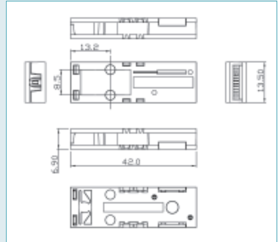
Compact Flat Manifold
