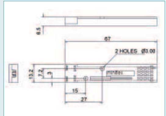
Long Flat Manifold
